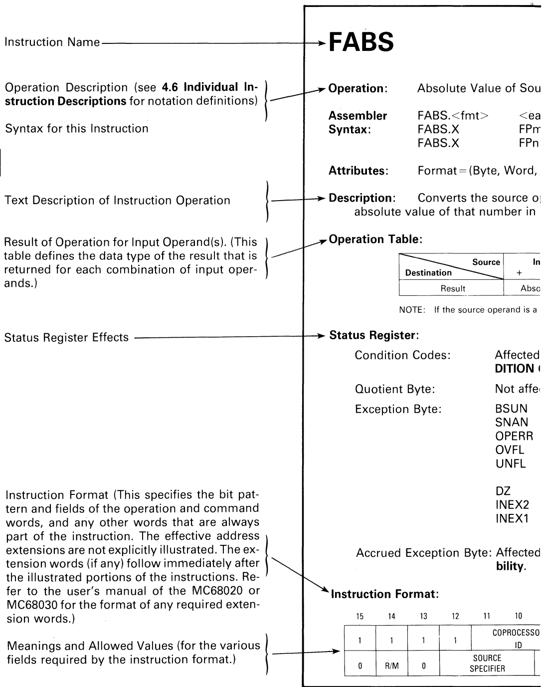
Figure 4-1. Instruction Description Format
