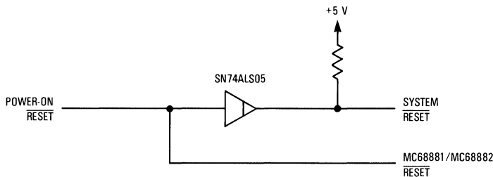
Figure 10-3. FPCP Reset Logic Example
