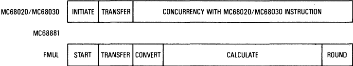
Figure 5-1. MC68881 Concurrency — FMUL Instruction
