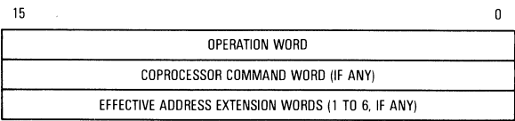
Figure 7-5. Coprocessor Instruction General Format
