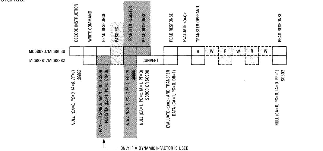
Figure 7-19. MC68882 External-to-Register Instruction Dialog
