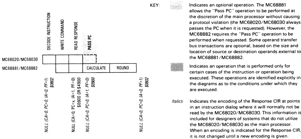
Figure 7-17. MC68881 Register-to-Register Instruction Dialog
