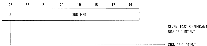
Figure 2-5. MC68881/MC68882 FPSR Quotient Byte
