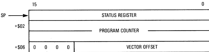
Figure 7-14. Pre-Instruction Exception Stack Frame
