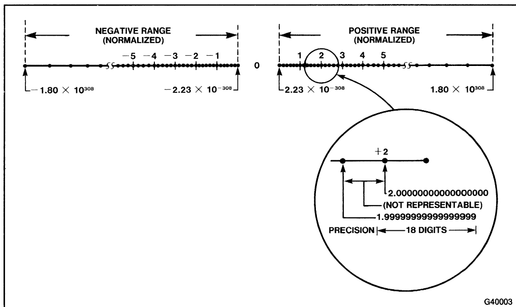
Figure 2-9. 80387 Double-Precision Number System
