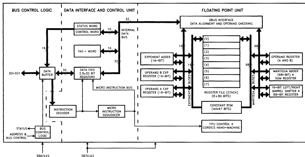
Figure 0.1. 80387 Block Diagram
