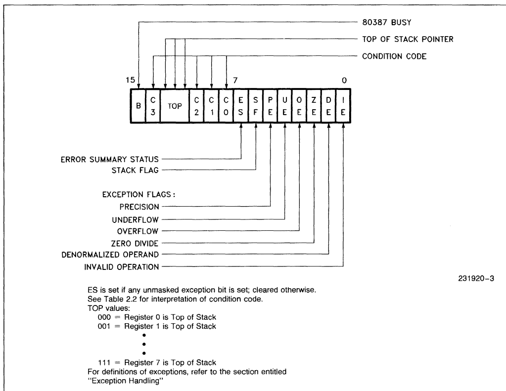
Figure 2.2. 80387 Status Word
