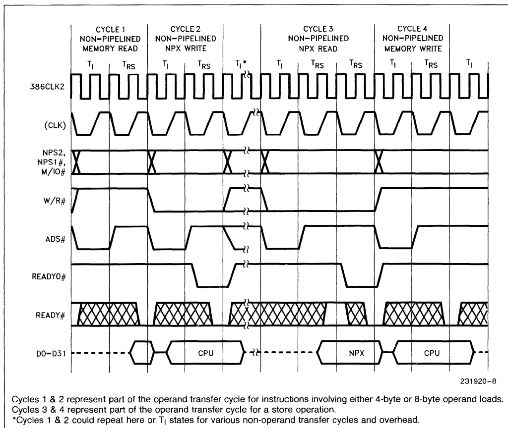
Figure 3.4. Nonpipelined Read and Write Cycles
