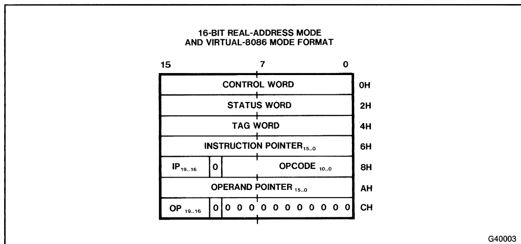
Figure 2-8. Real Mode 80387 Instruction and Data Pointer Image in Memory, 16-Bit Format
