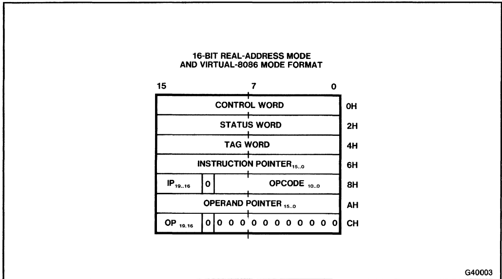
Figure 4-6. Real Mode 80387 Environment, 16-Bit Format
