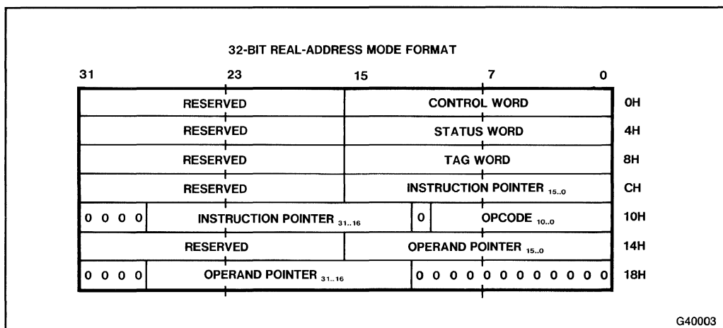
Figure 2-6. Real Mode 80387 Instruction and Data Pointer Image in Memory, 32-Bit Format
