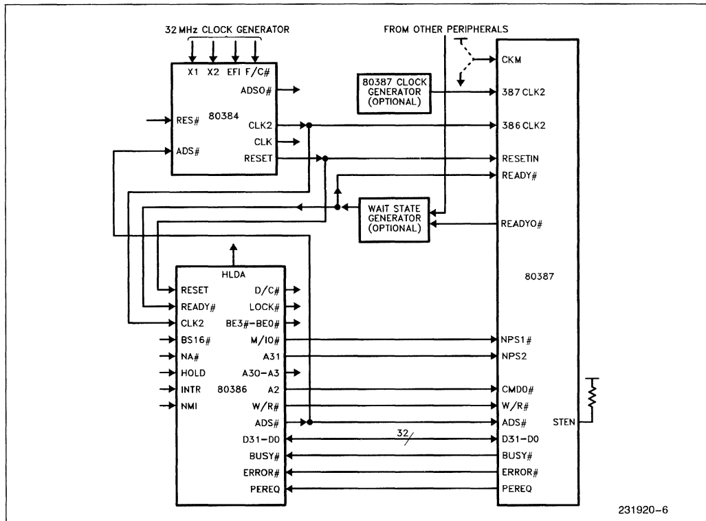
Figure 3.2. 80386/80387 System Configuration
