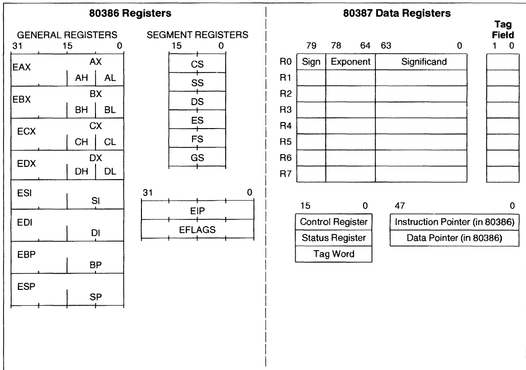
Figure 1.1. 80386/80387 Register Set
