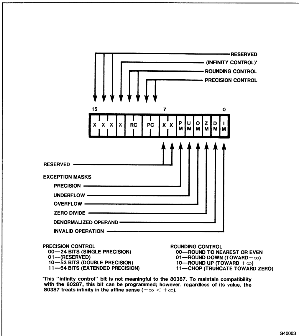
Figure 2-3. 80387 Control Word Format
