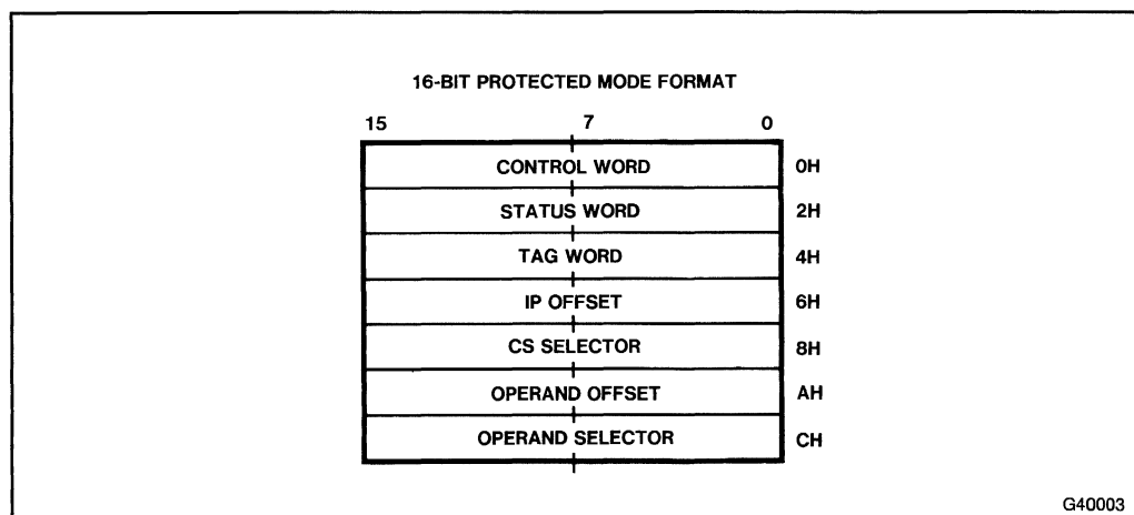
Figure 4-5. Protected Mode 80387 Environment, 16-Bit Format
