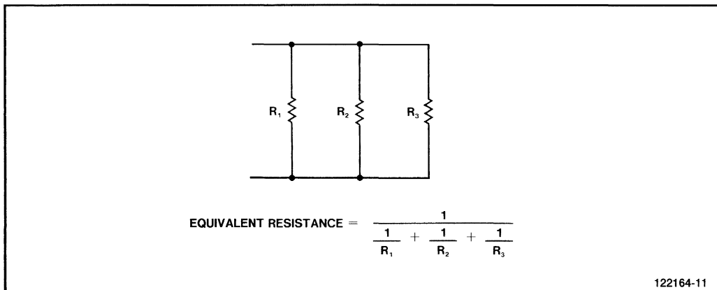
Figure 3-3. Arithmetic Example Using Infinity
