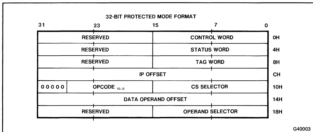
Figure 2-5. Protected Mode 80387 Instruction and Data Pointer Image in Memory, 32-Bit Format
