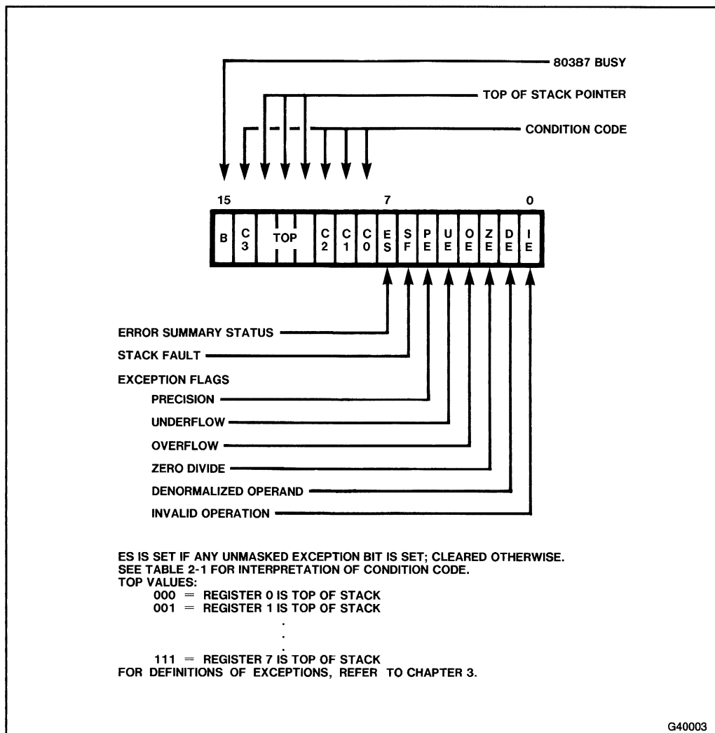
Figure 2-2. 80387 Status Word
