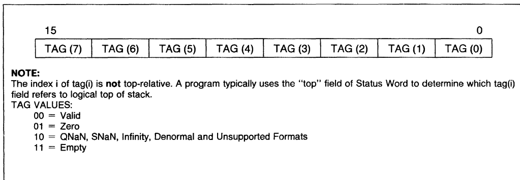
Figure 2.1. 80387 Tag Word
