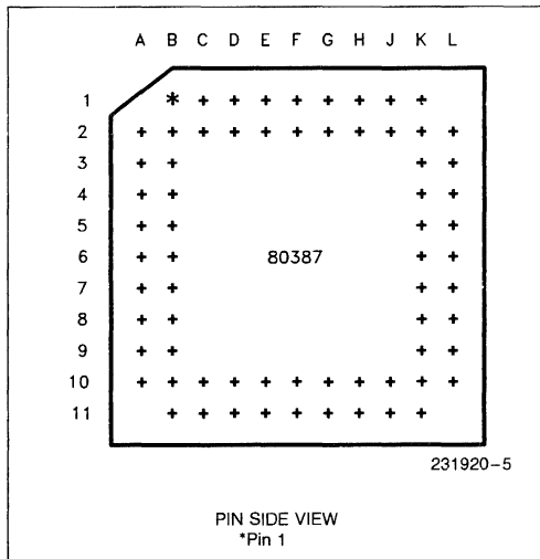
Figure 3.1. 80387 Pin Configuration
