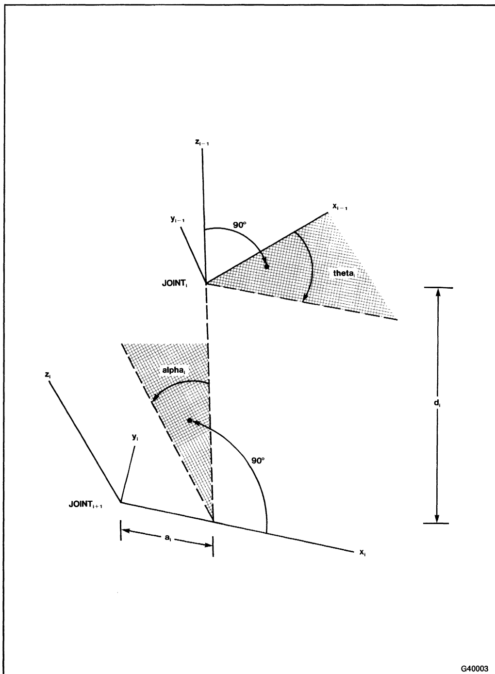
Figure 7-7. Relationships between Adjacent Joints
