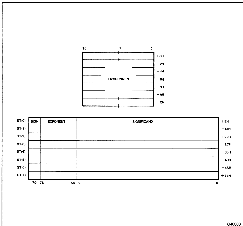
Figure 4-2. FSAVE/FRSTOR Memory Layout (16-Bit)
