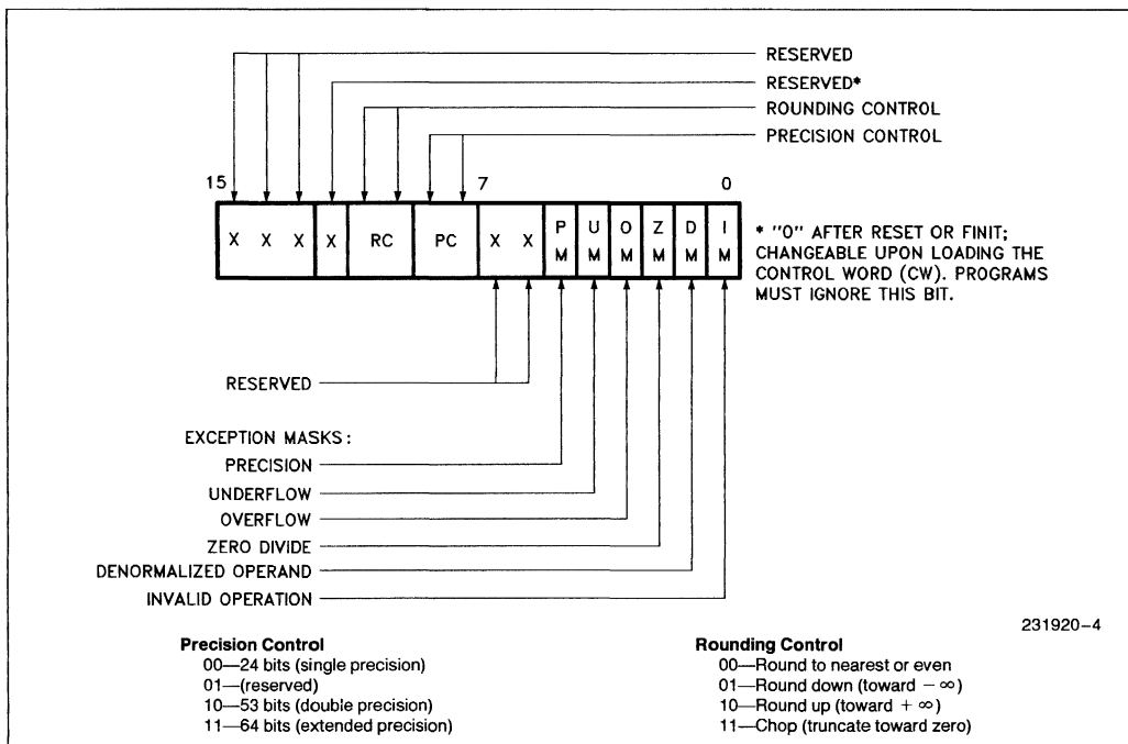
Figure 2.7. 80387 Control Word
