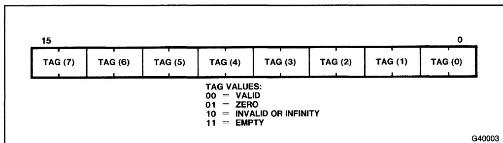
Figure 2-4. 80387 Tag Word Format
