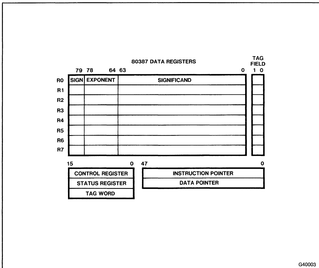
Figure 2-1. 80387 Register Set
