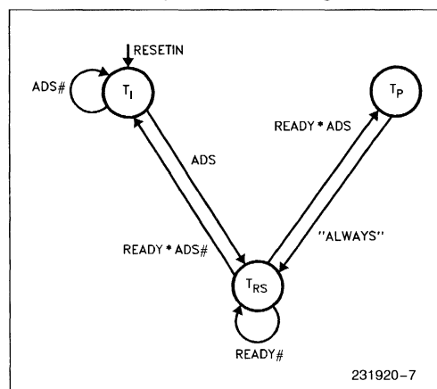
Figure 3.3. Bus State Diagram
