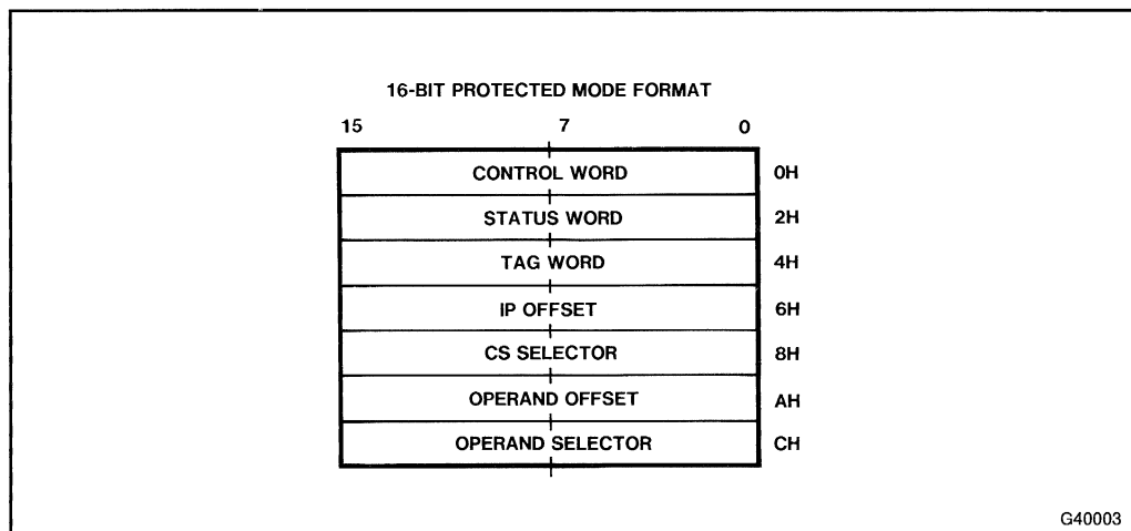
Figure 2-7. Protected Mode 80387 Instruction and Data Pointer Image in Memory, 16-Bit Format
