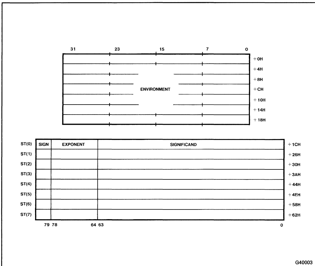
Figure 4-1. FSAVE/FRSTOR Memory Layout (32-Bit)
