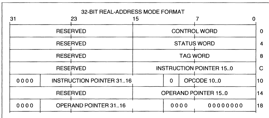
Figure 2.4. Real Mode 80387 Instruction and Data Pointer Image in Memory, 32-Bit Format
