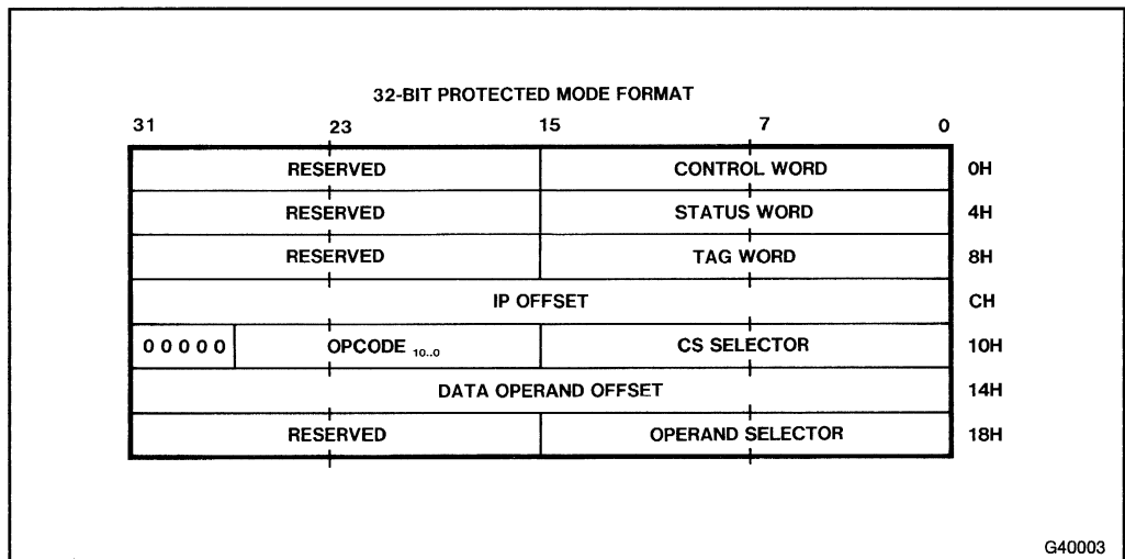
Figure 4-3. Protected Mode 80387 Environment, 32-Bit Format
