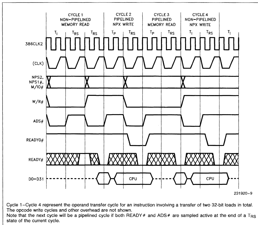
Figure 3.5. Fastest Transitions to and from Pipelined Cycles
