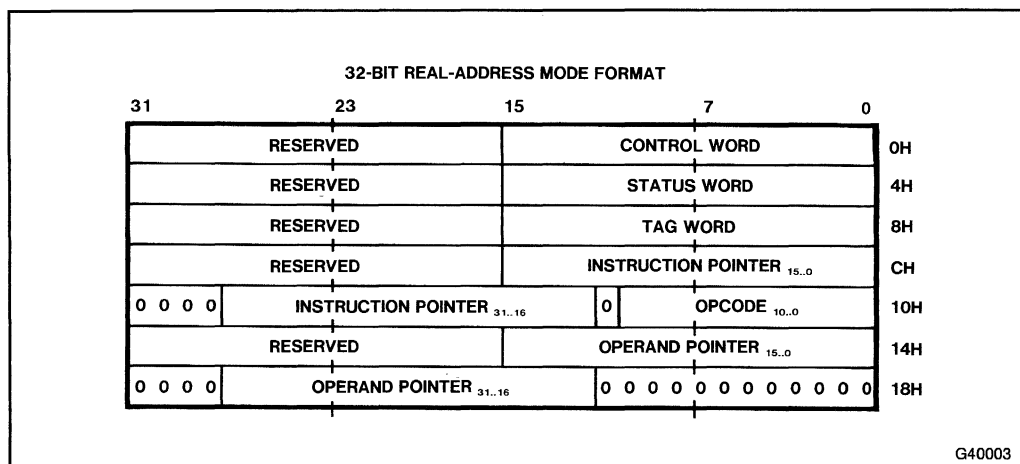
Figure 4-4. Real Mode 80387 Environment, 32-Bit Format
