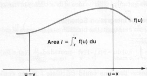
Fig. 1. An integral interpreted as an area.
